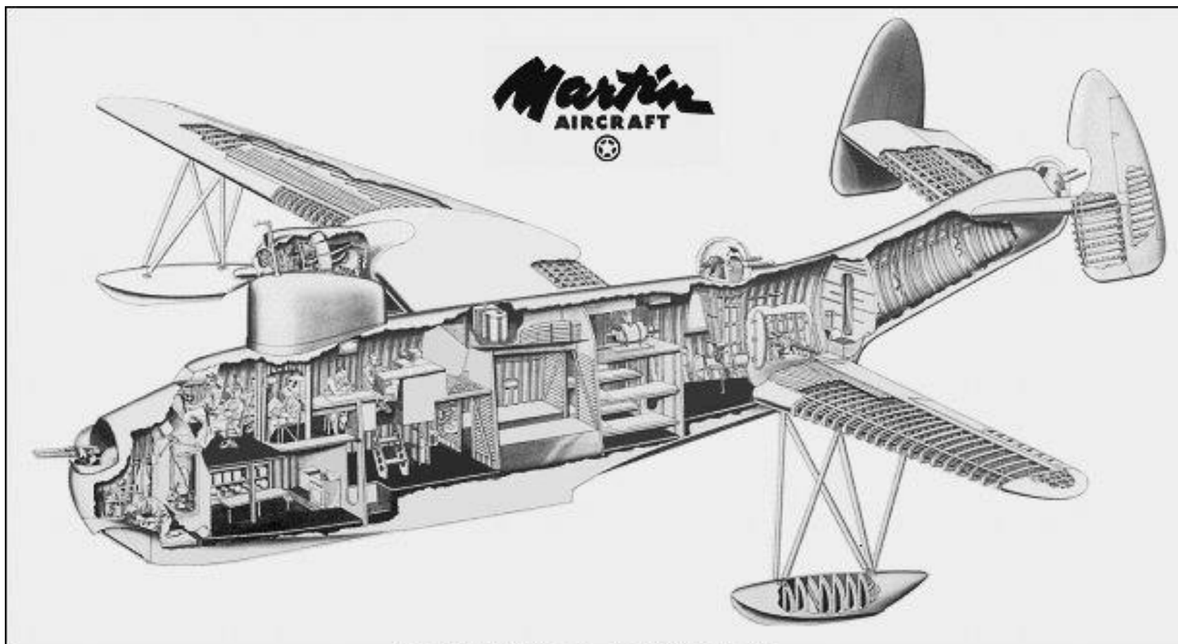
PBM-5 MARINER (MARTIN)
